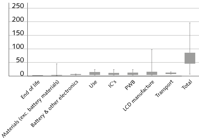
GWP impact/product (kg CO 2 eq)
